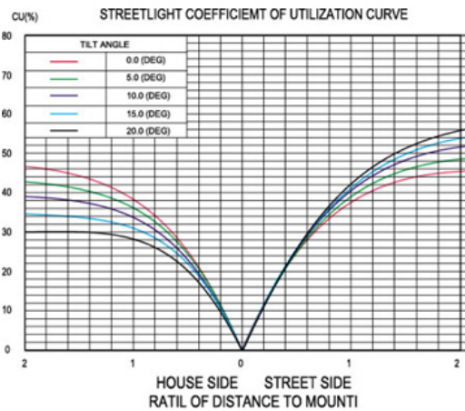
2. UTILIZATION FACTORS
