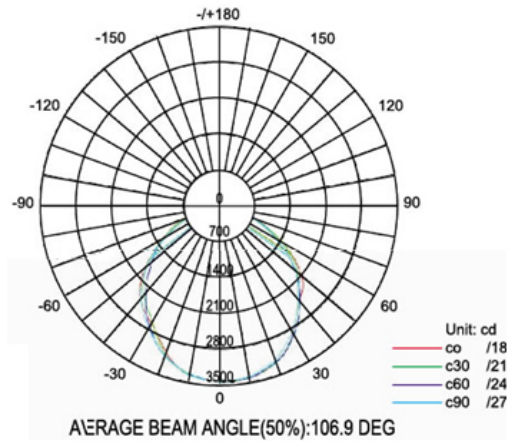
1. POLAR DIAGRAM
