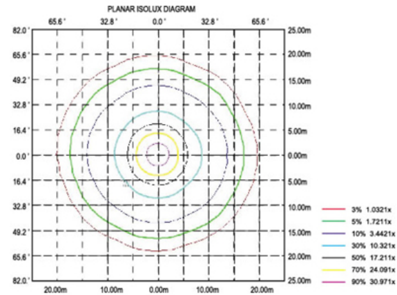
4. ISOLUX DIAGRAM
